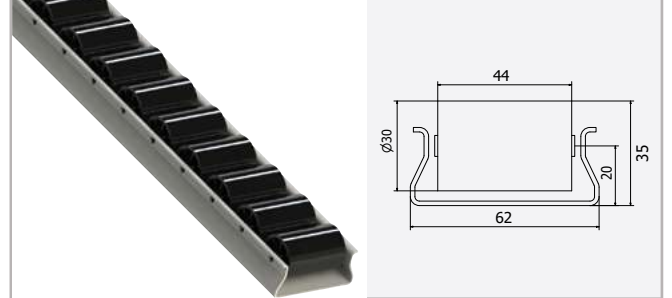
CVRT-15 - PP Makara
