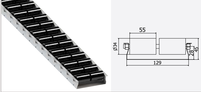
CVRT-12 - PP Makara
